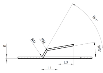
Z-Lasche / without crinkle
