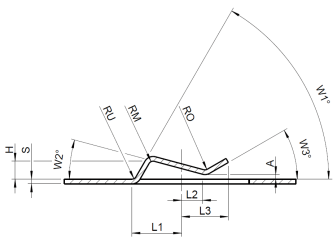
Klemmlasche / with crinkle
